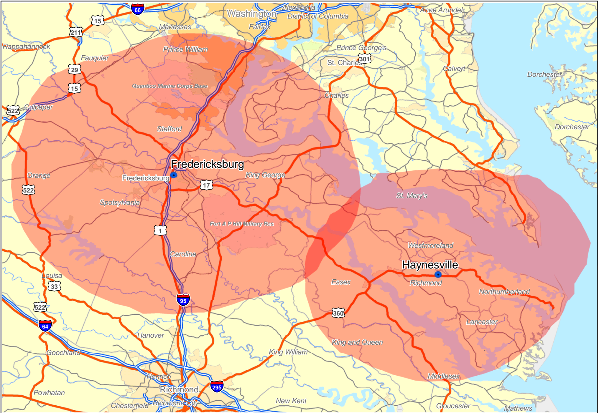
Virginia Regional MOTOTRBO Coverage
